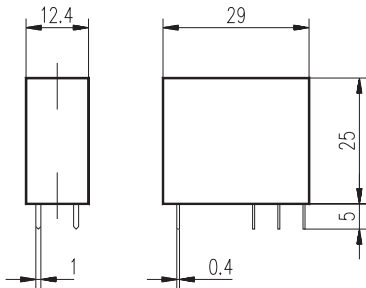
fig. 2 relay 2 change-over contacts
