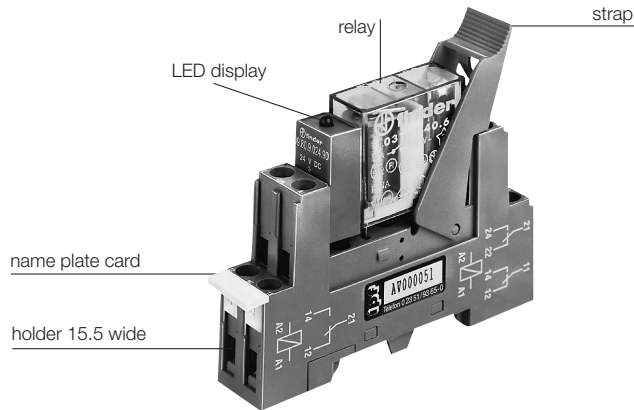
relay connection
