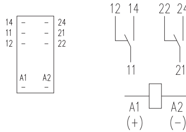
relay connection
