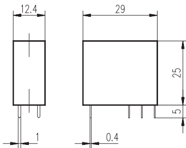
fig. 1 relay 1 change-over contact
