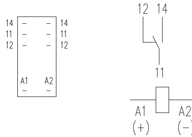
relay connection
