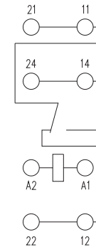
holder connection
